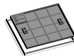
Modelo rectangular Rectangular model EPAL 700x500
